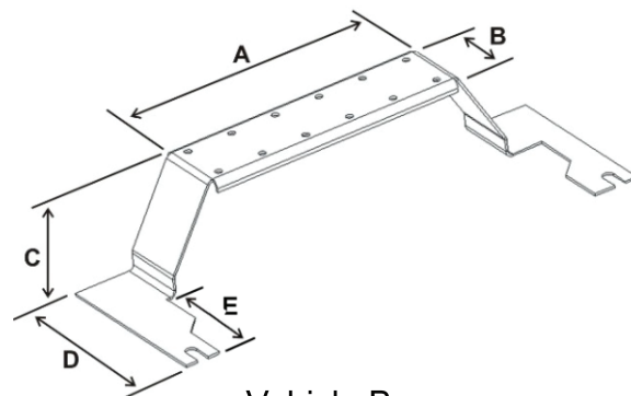
Vehicle Base RAM-VB-103
